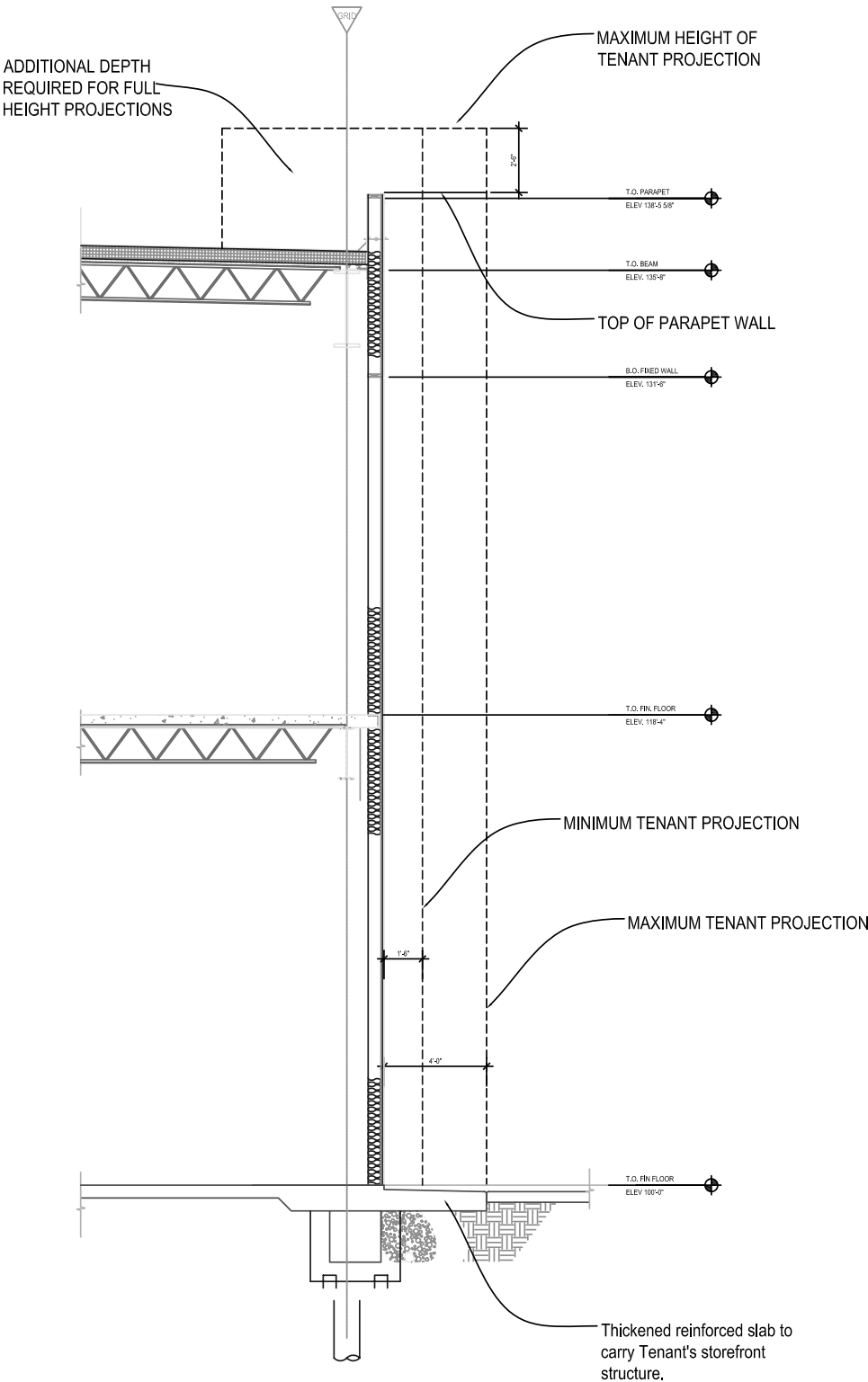
EXTERIOR SECTION NTS
