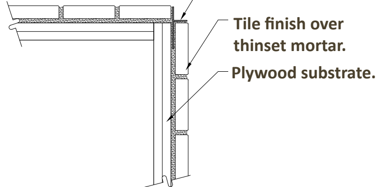
CORNER DETAIL
