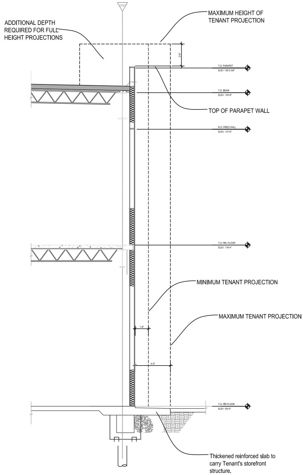
EXTERIOR SECTION NTS
