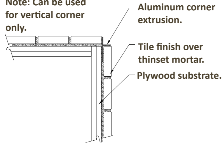
CORNER DETAIL
