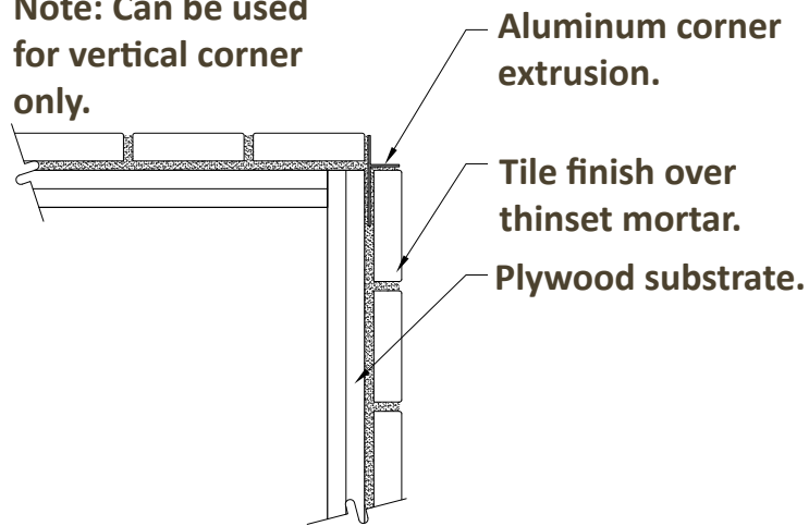
CORNER DETAIL
