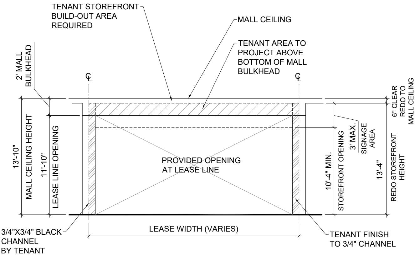
Lower Level Storefront Elevation
