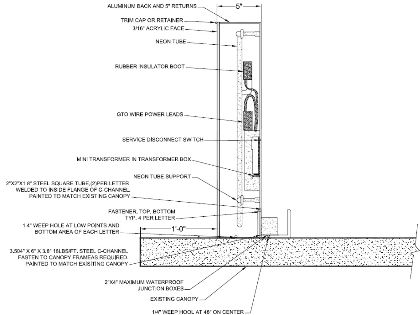
Self-contained 20"-36" high pan channel LED illuminated letters
