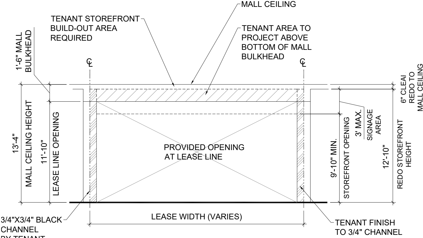
UPPER LEVEL STOREFRONT ELEVATION
