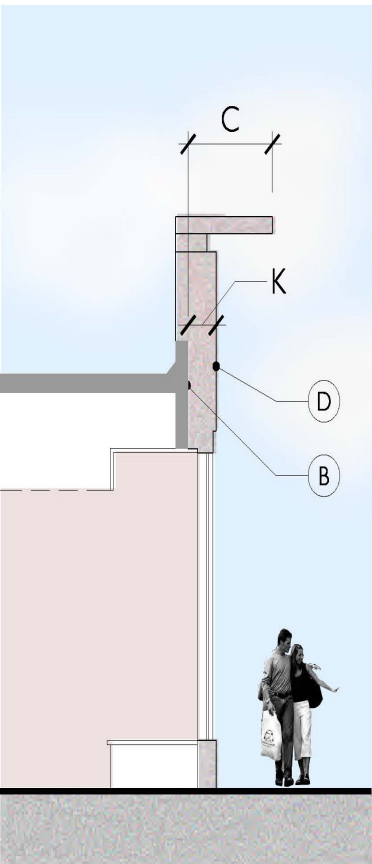
Arcade Section
