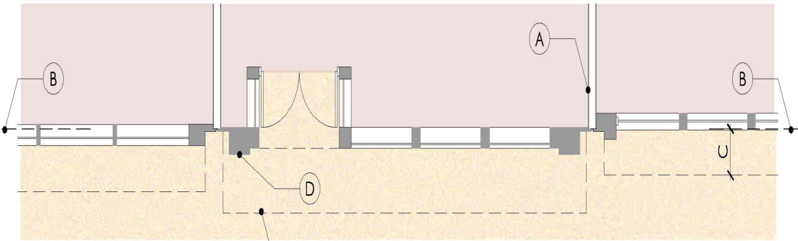
Arcade Plan
