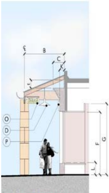
Arcade Section
