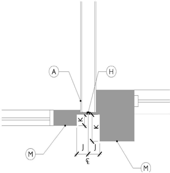
Demising Wall Detail
