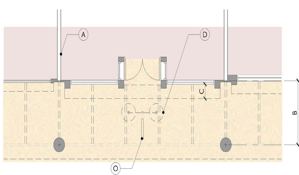
Arcade Plan
