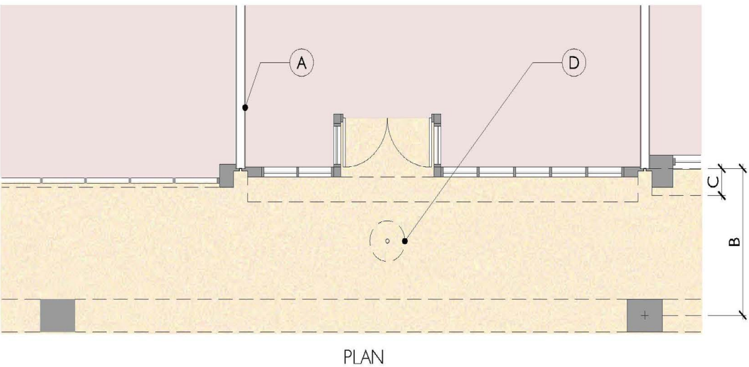
Arcade Plan
