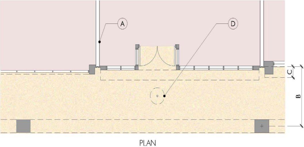
Arcade Plan
