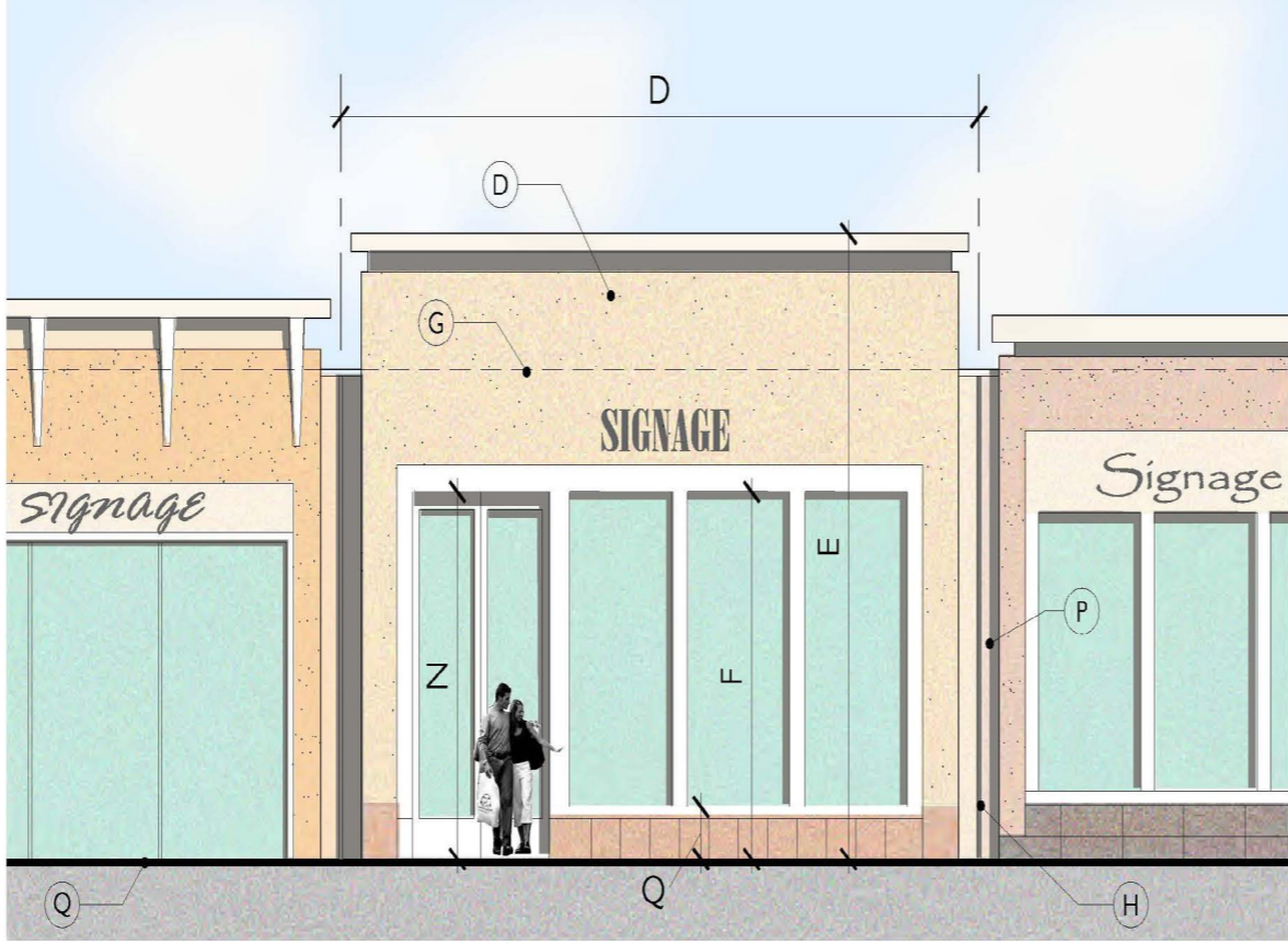
Storefront Elevation
