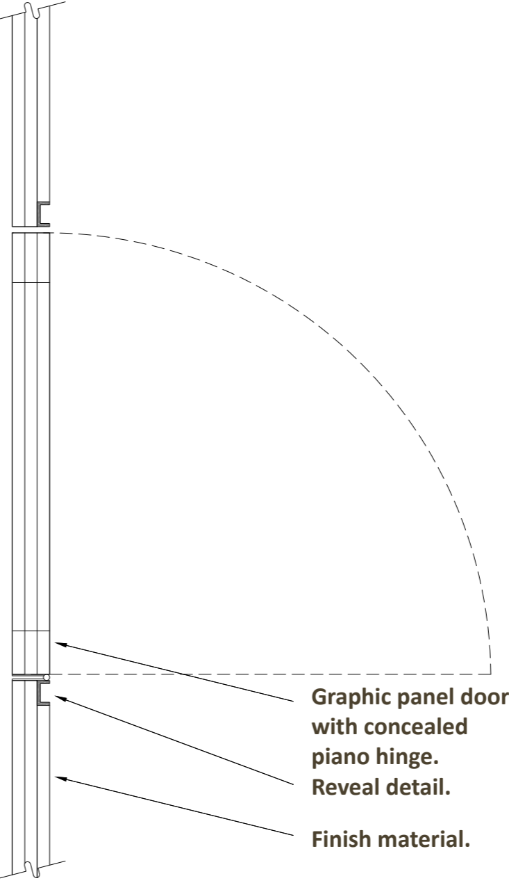
GRAPHIC FRAME DETAIL
