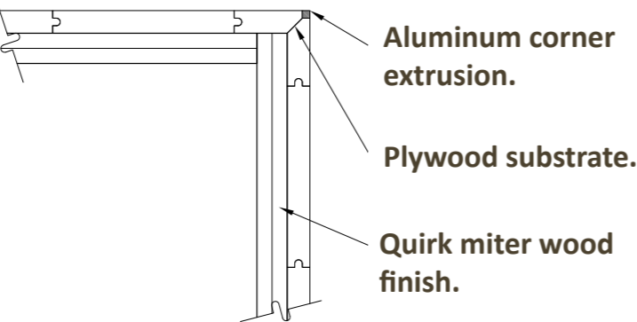
CORNER DETAIL
