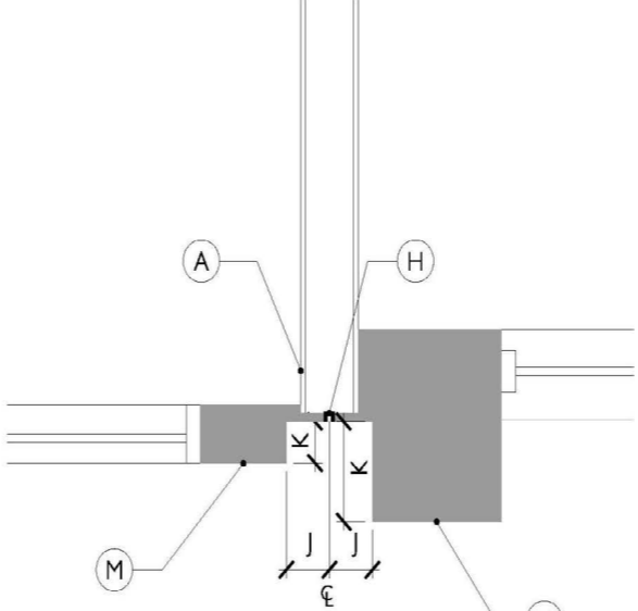
Demising Wall Detail
