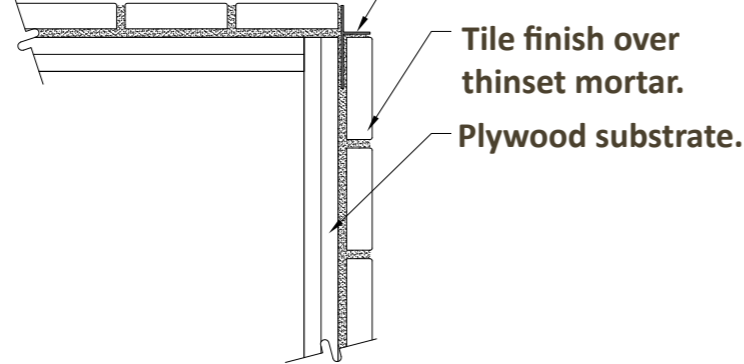
CORNER DETAIL
