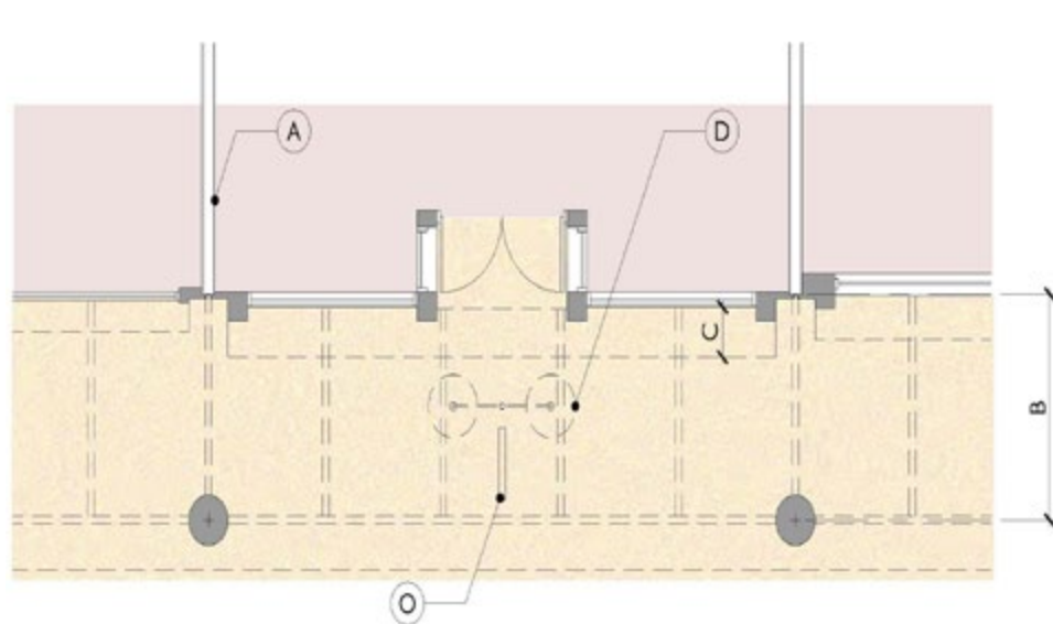
Arcade Plan
