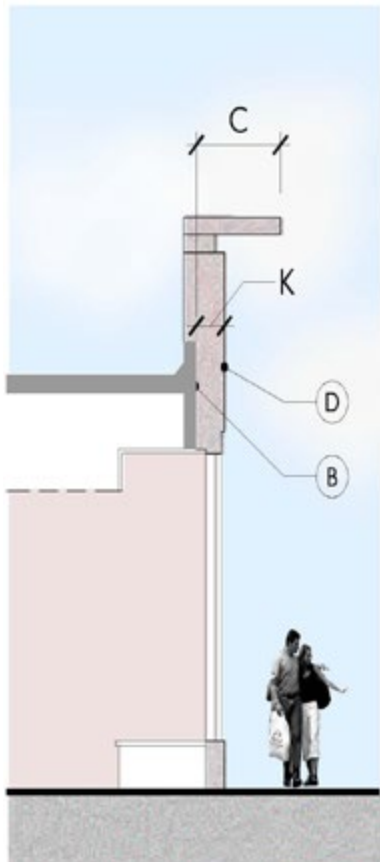
Arcade Section
