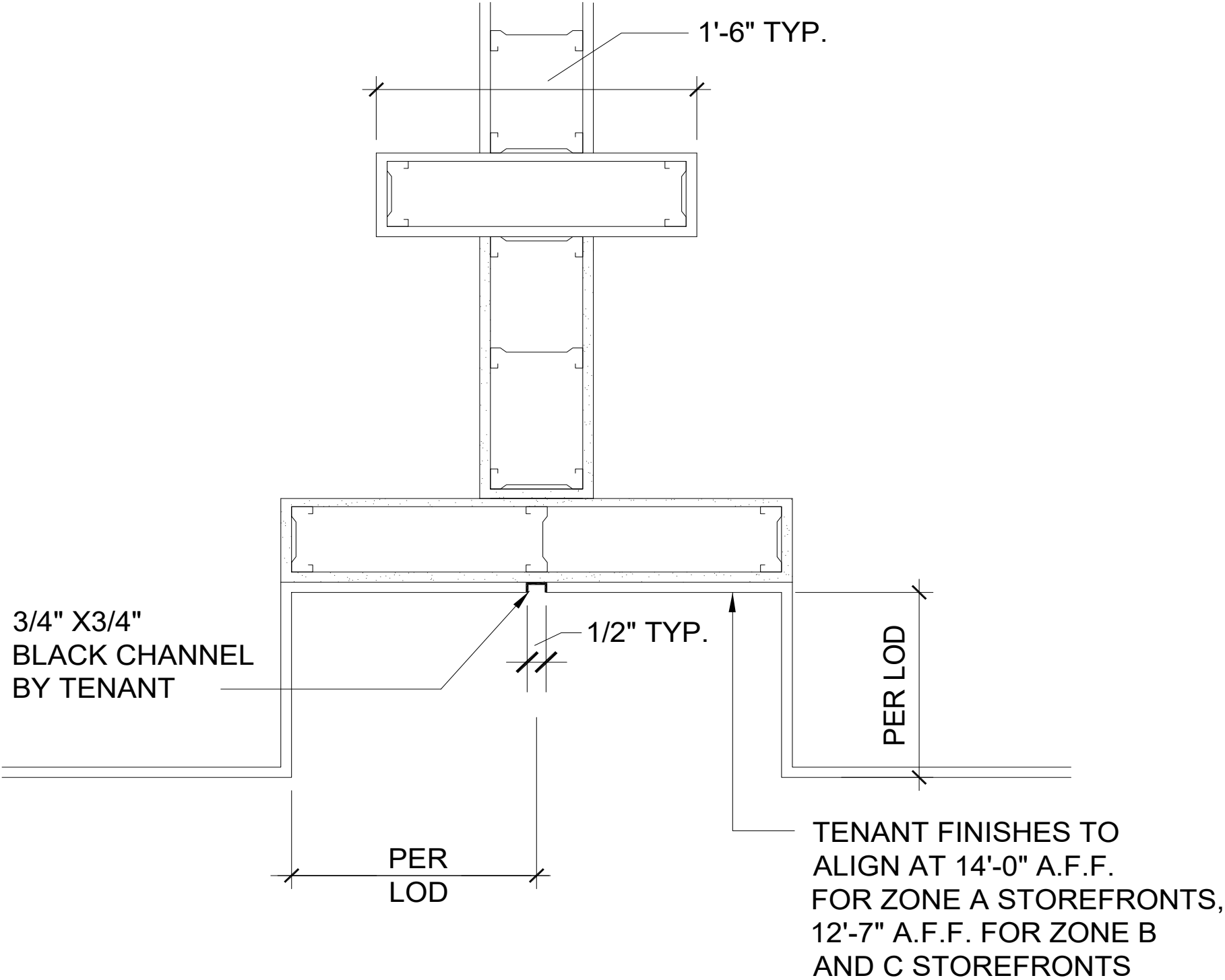
TYPICAL NEUTRAL PIER CONTACT MALL T.C. FOR MORE INFORMATION - N.T.S.
