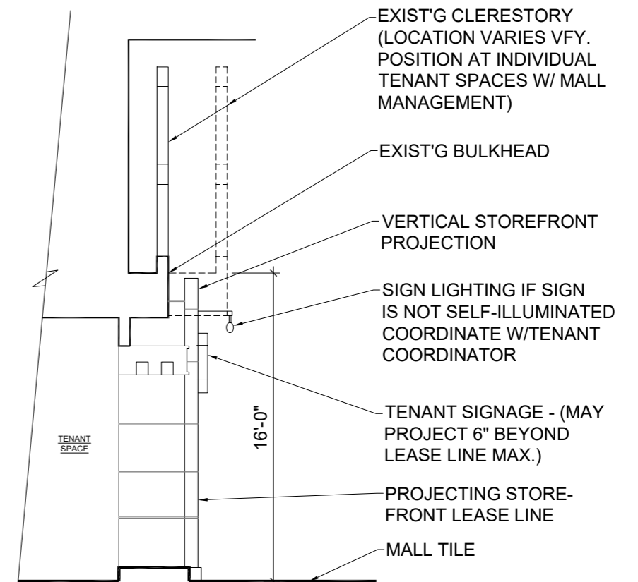
TYPICAL SECTION DETAIL - ZONE A CONTACT MALL T.C. FOR MORE INFORMATION - N.T.S.
