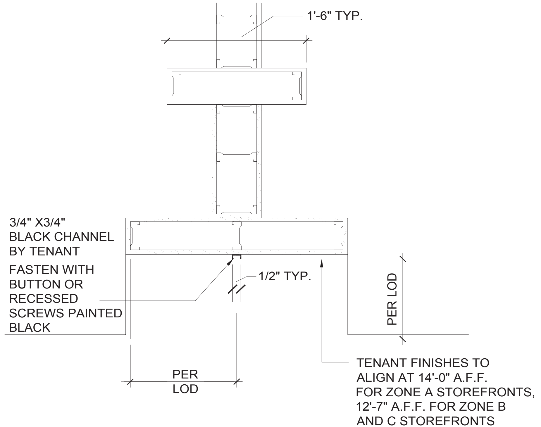
TYPICAL NEUTRAL PIER CONTACT MALL T.C. FOR MORE INFORMATION - N.T.S.
