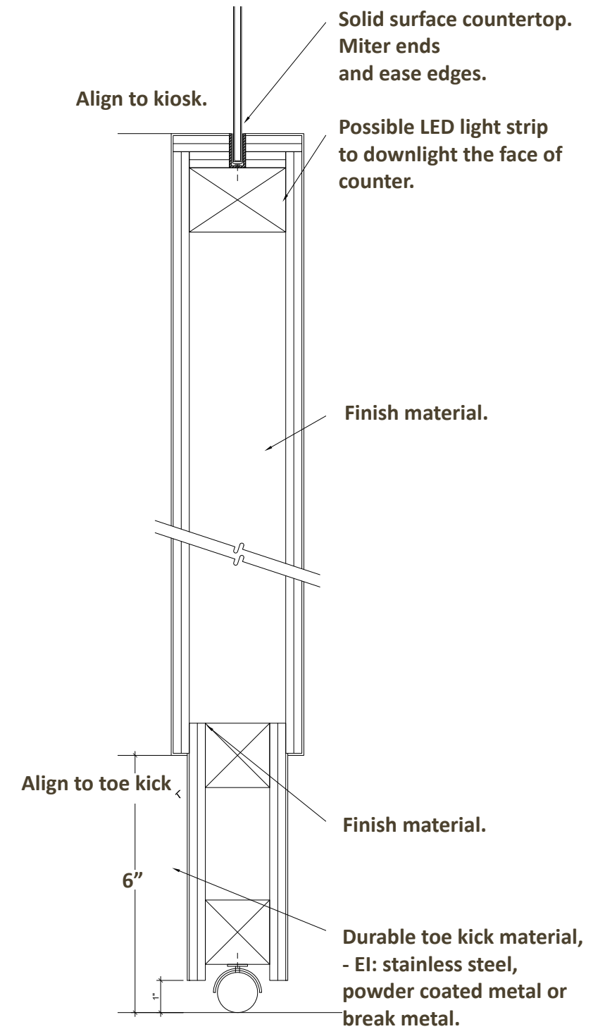
GATE DETAIL
