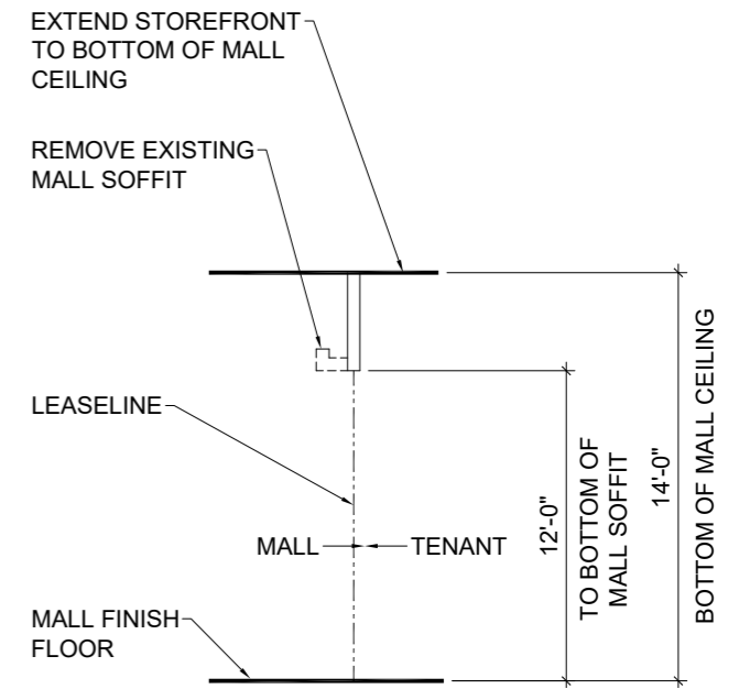
TYPICAL SECTION DETAIL CONTACT MALL T.C. FOR MORE INFORMATION - N.T.S.
