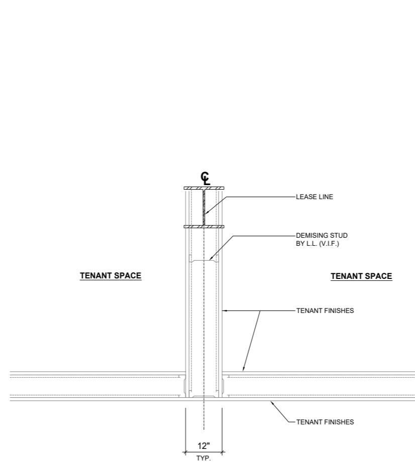
TYPICAL NEUTRAL PIER DETAIL CONTACT MALL T.C. FOR MORE INFORMATION - N.T.S.
