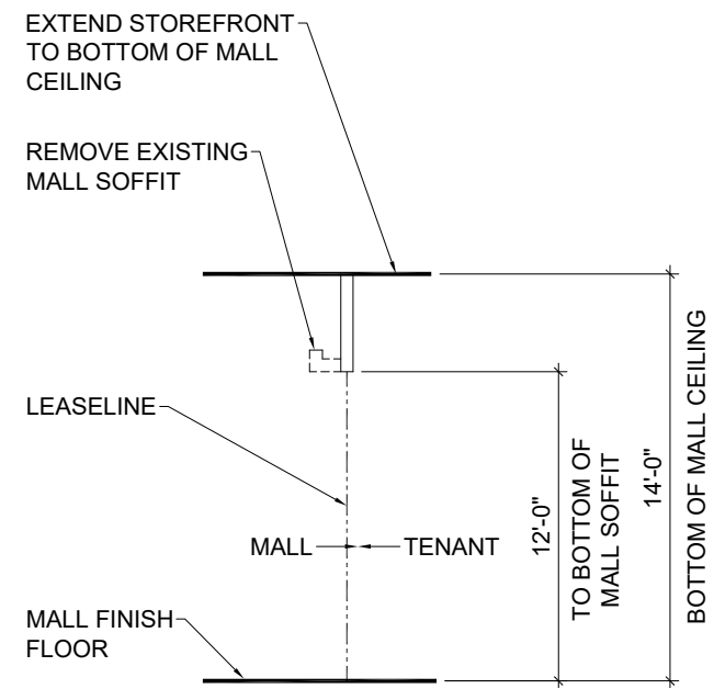
TYPICAL SECTION DETAIL CONTACT MALL T.C. FOR MORE INFORMATION - N.T.S.
