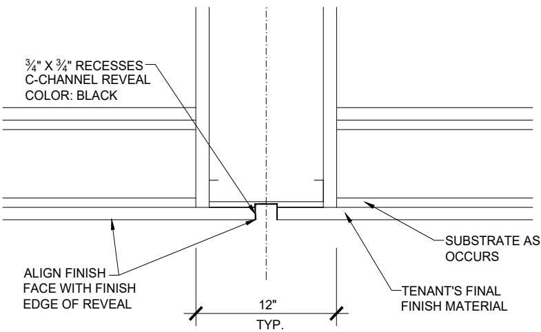
TYPICAL NEUTRAL PIER DETAIL- CLOSE UP CONTACT MALL T.C. FOR MORE INFORMATION - N.T.S.
