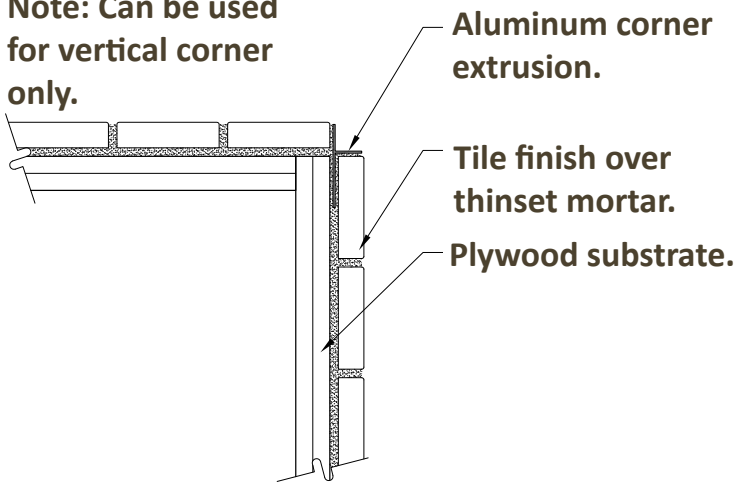
CORNER DETAIL
