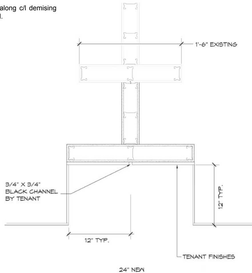
PLAN DETAIL @ NEUTRAL CHANNEL CONDITION SCALE: NTS
