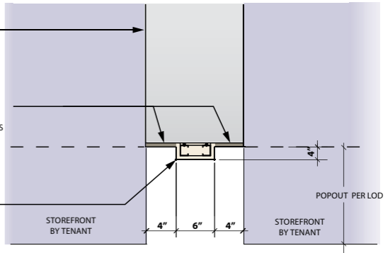
AREA E NEUTRAL PIER PLAN VIEW SCALE: NTS
