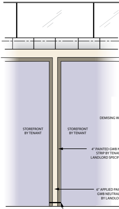
AREA E NEUTRAL PIER ELEVATION SCALE: NTS
