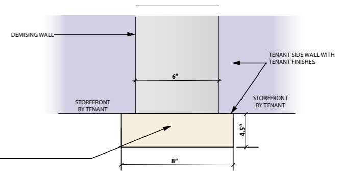
B - AREA C NEUTRAL PIER PLAN VIEW SCALE: NTS
