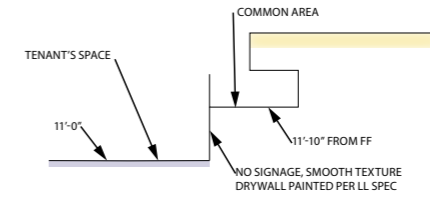
A - AREA C SECTION AT BULKHEAD SCALE: NTS
