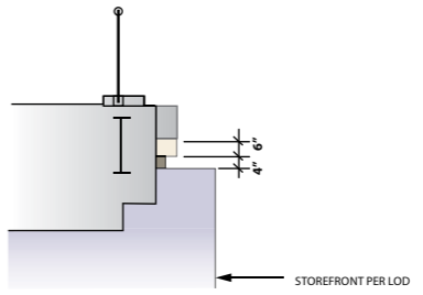
AREA D SECTION AT BULKHEAD SCALE: NTS
