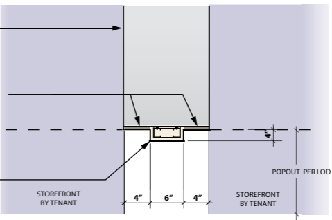
AREA D NEUTRAL PIER PLAN VIEW SCALE: NTS
