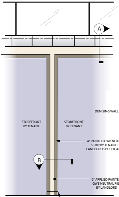
AREA D NEUTRAL PIER ELEVATION SCALE: NTS
