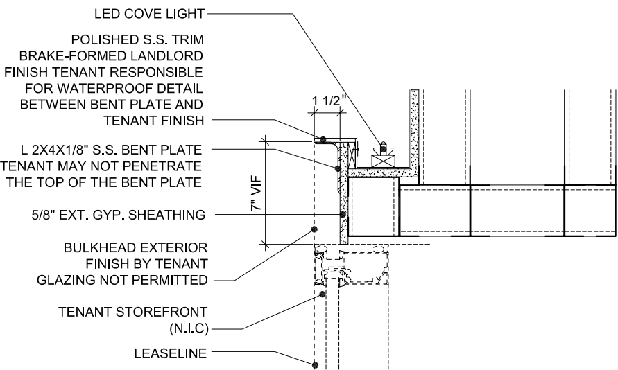
HEAD DETAIL
