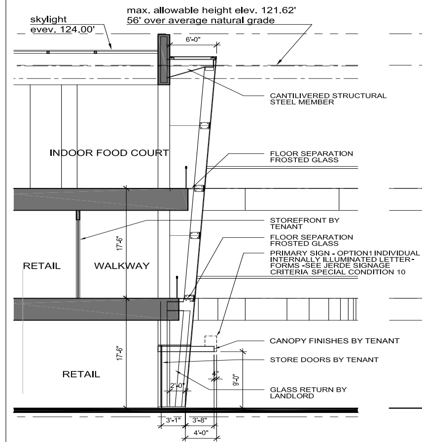
SECTION
