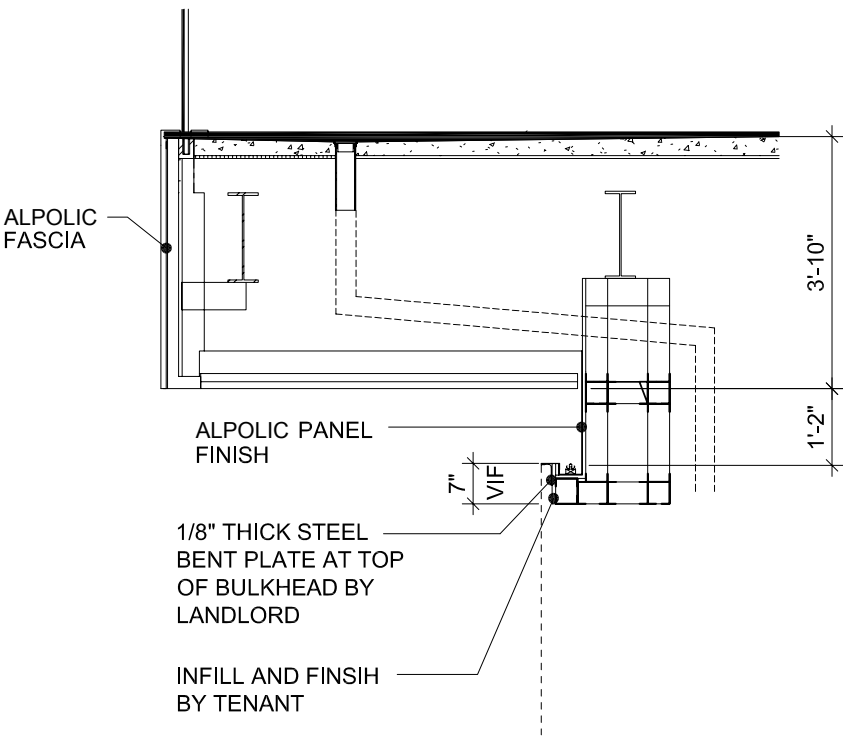
DETAIL SECTION
