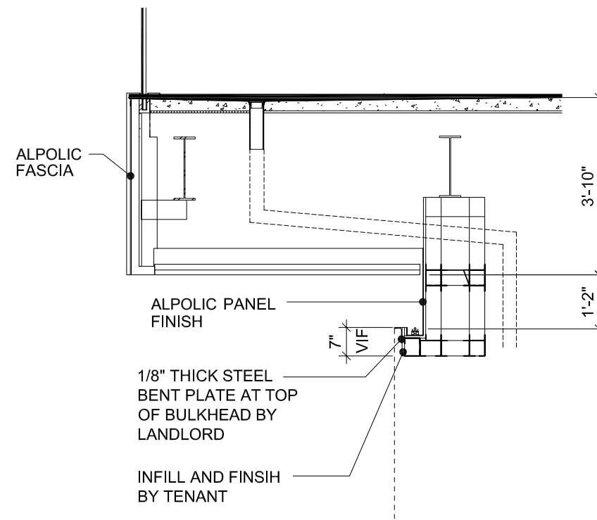
DETAIL SECTION
