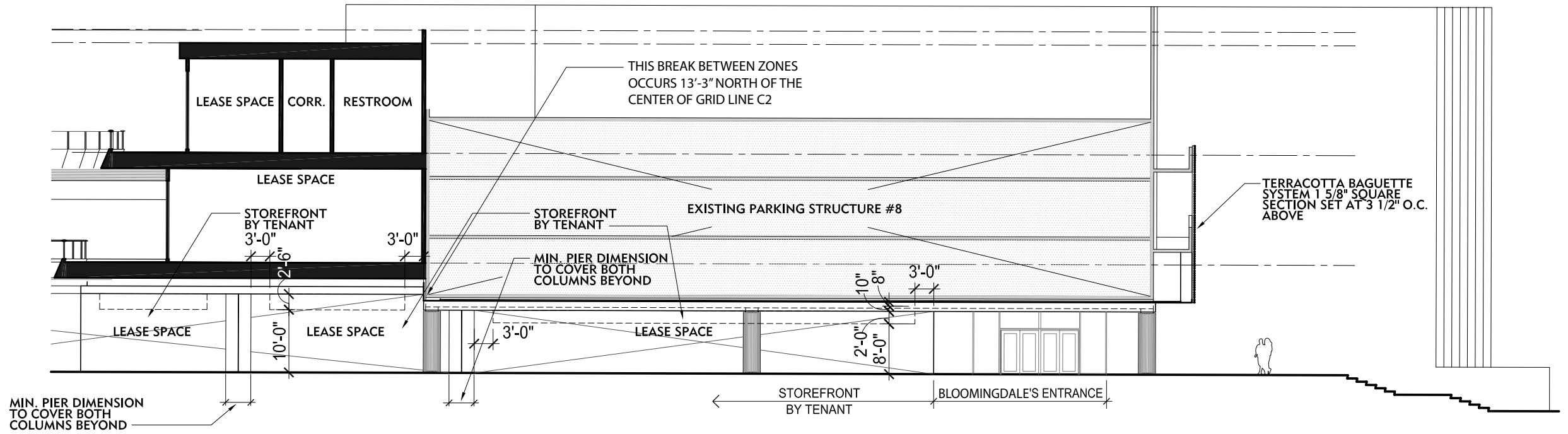
EAST ELEVATION
