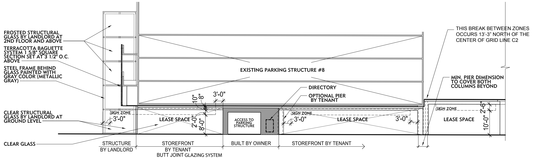
WEST ELEVATION
