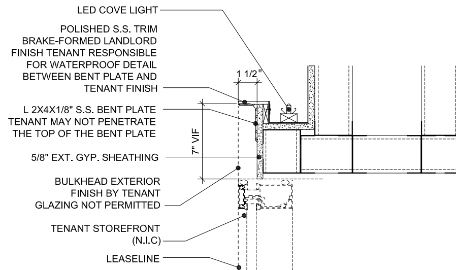
HEAD DETAIL
