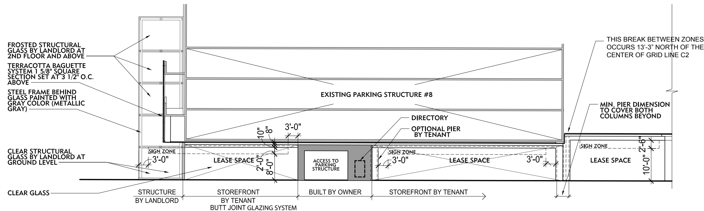
WEST ELEVATION
