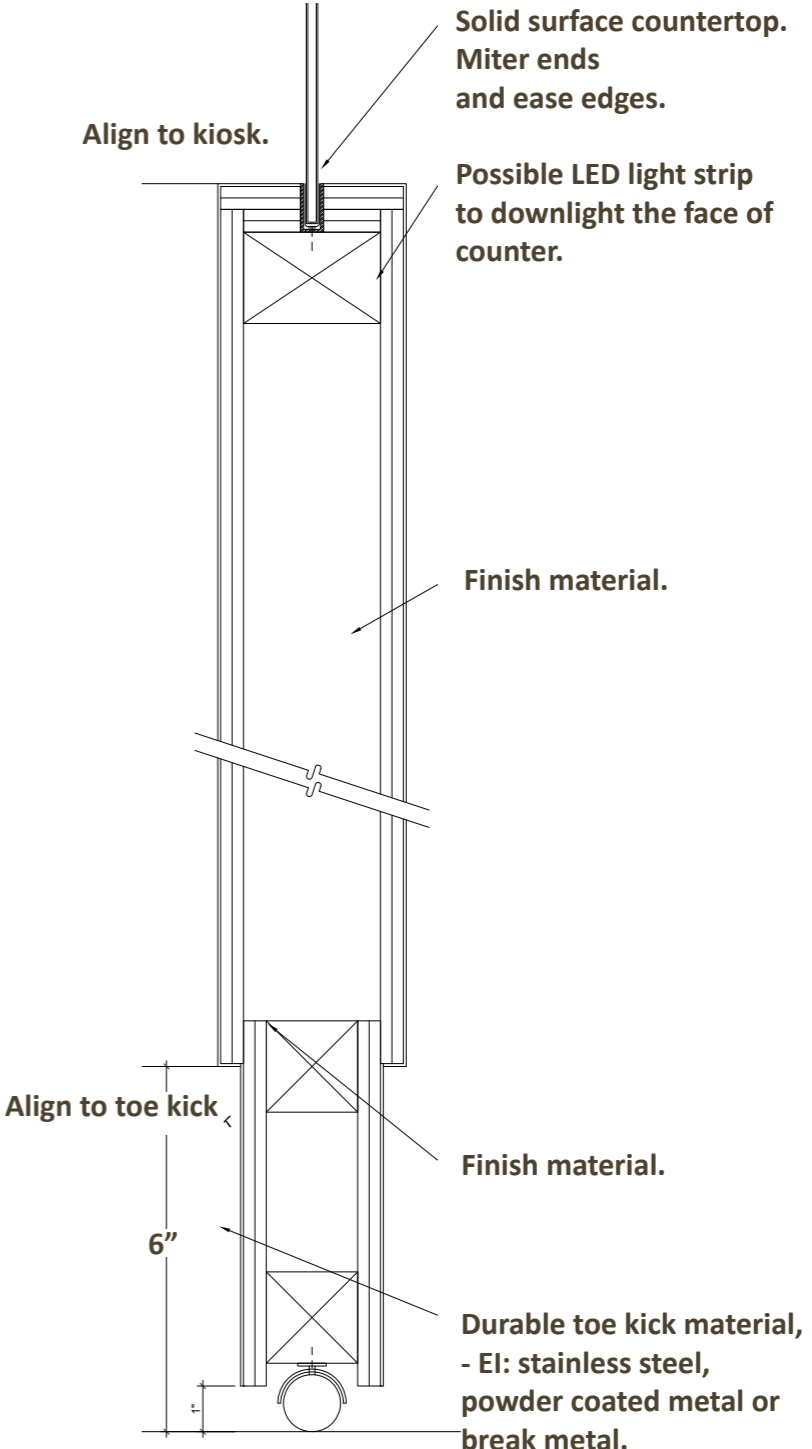
GATE DETAIL
