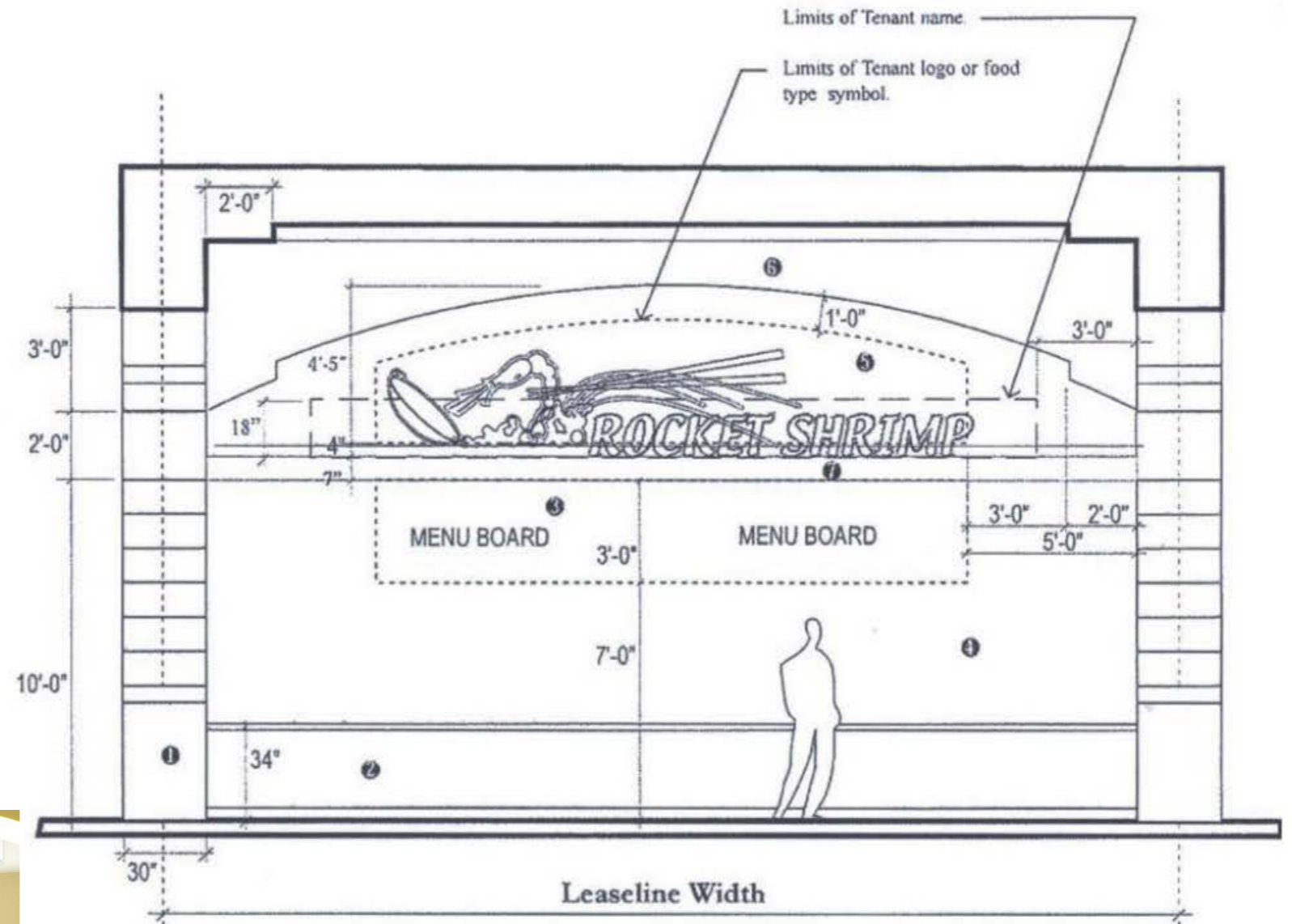
TYPICAL TENANT COUNTER ELEVATION.
