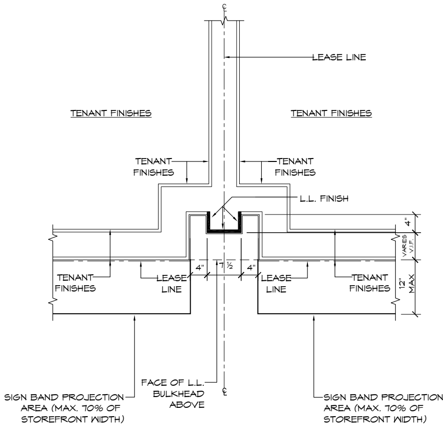
PROPOSED NEUTRAL PIER DTL.
