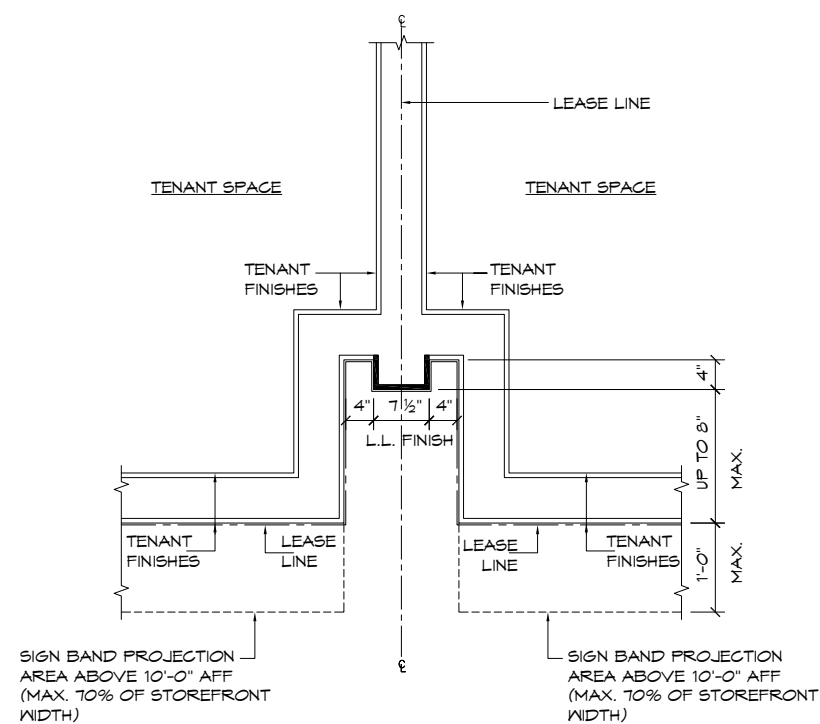
PROPOSED NEUTRAL PIER DTL.
