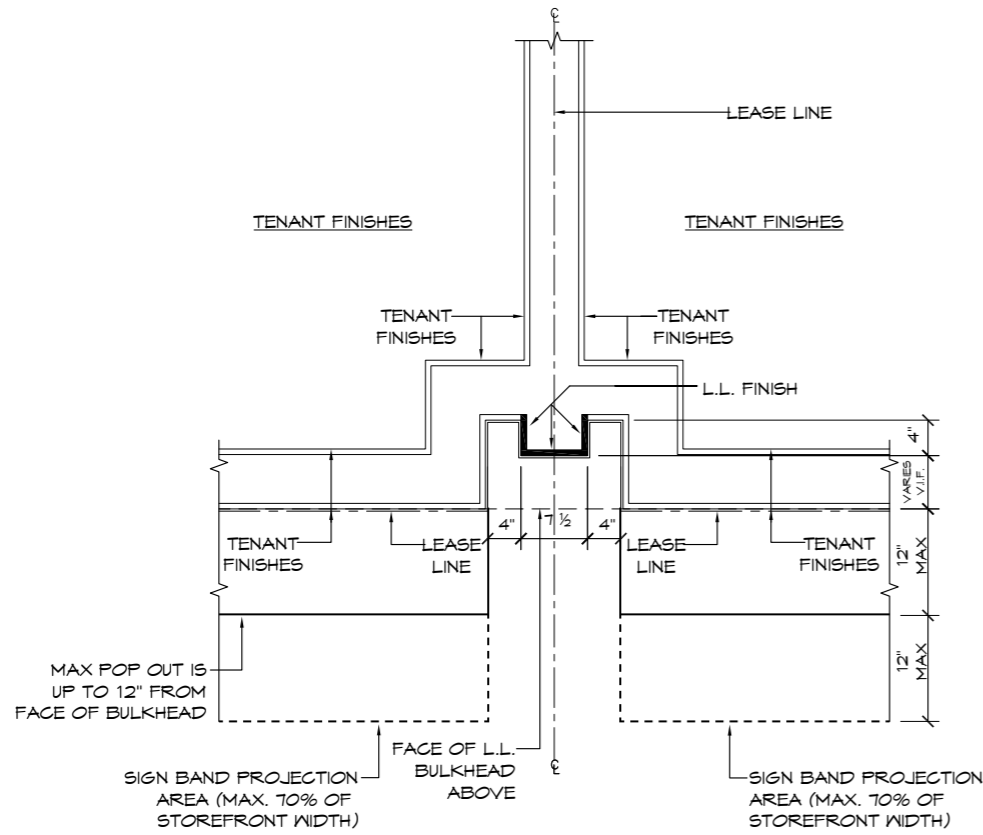
PROPOSED NEUTRAL PIER DTL.
