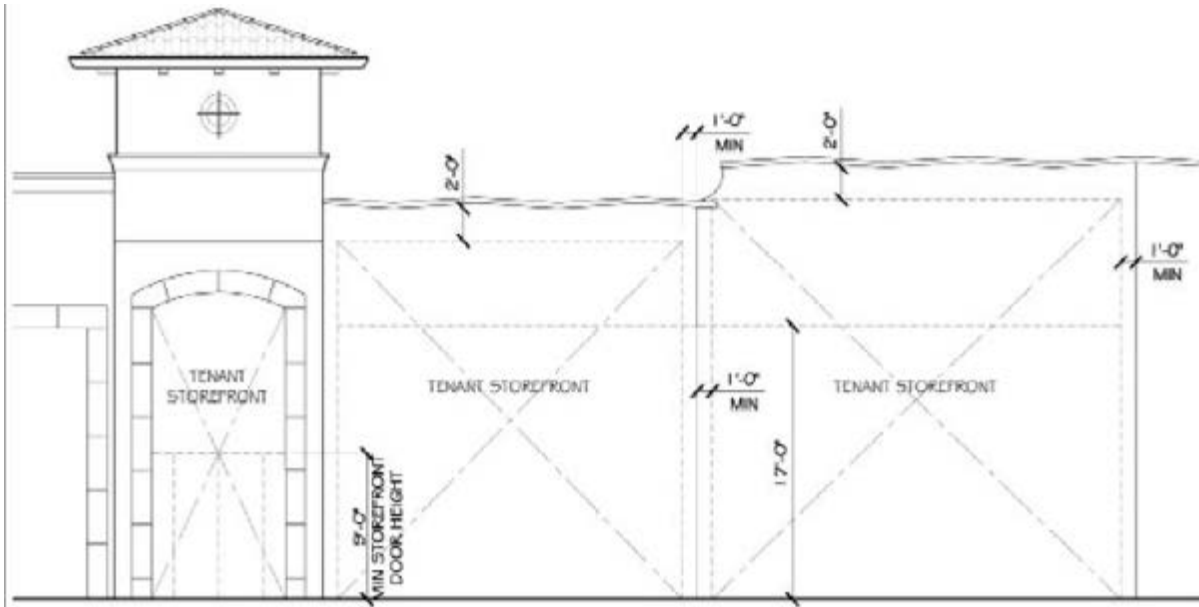
ELEVATION DETAIL
