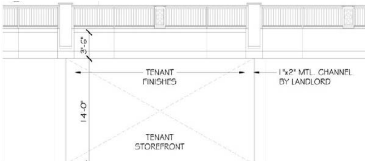
ELEVATION DETAIL
