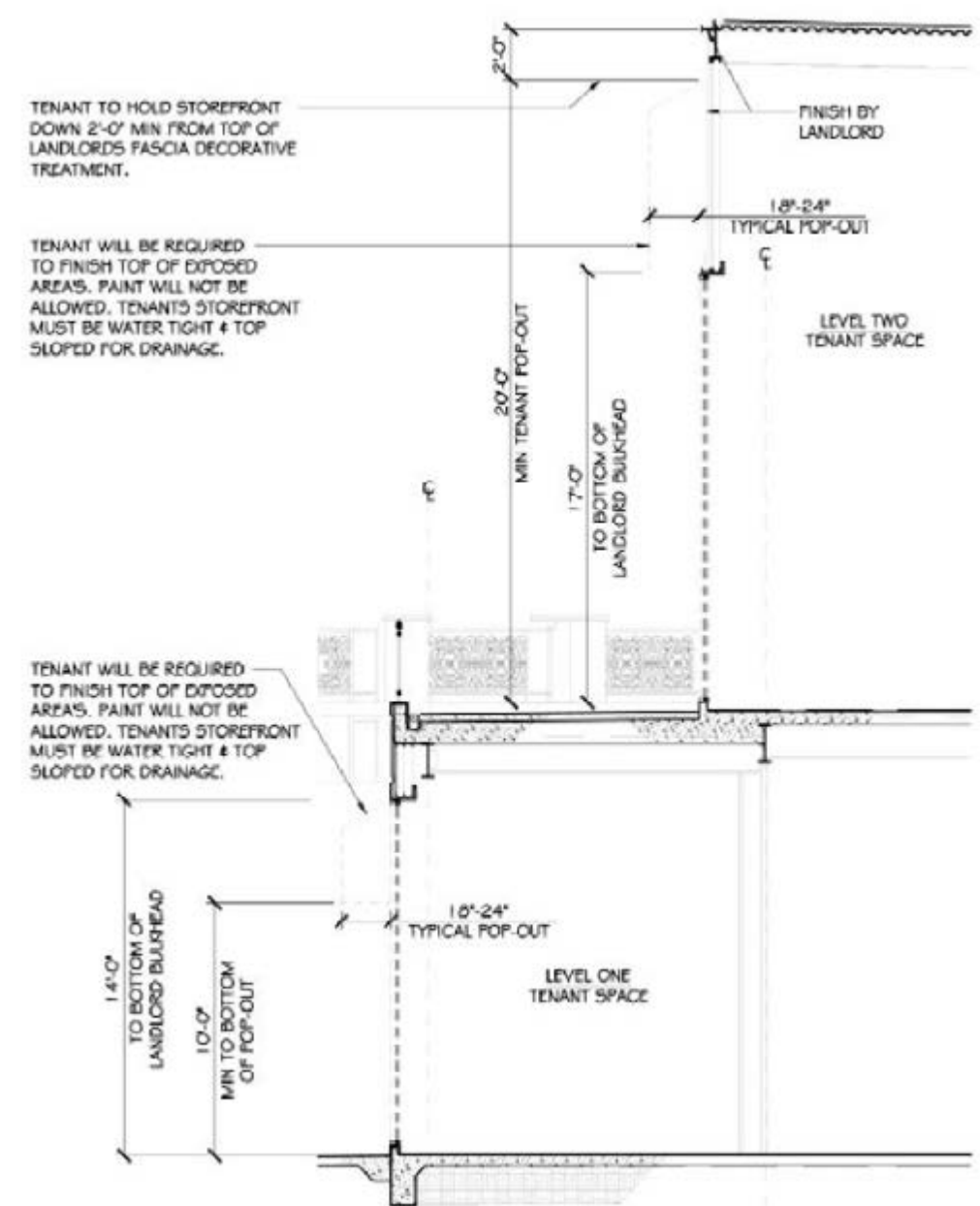
SECTION DETAIL
