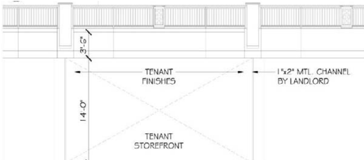
ELEVATION DETAIL
