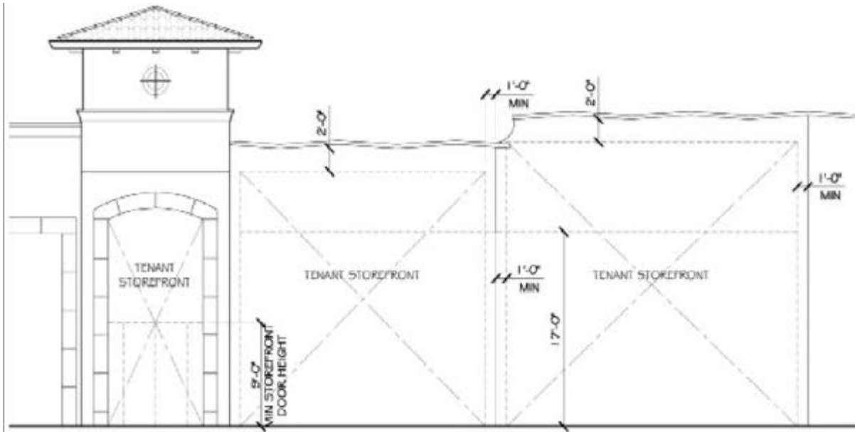
ELEVATION DETAIL
