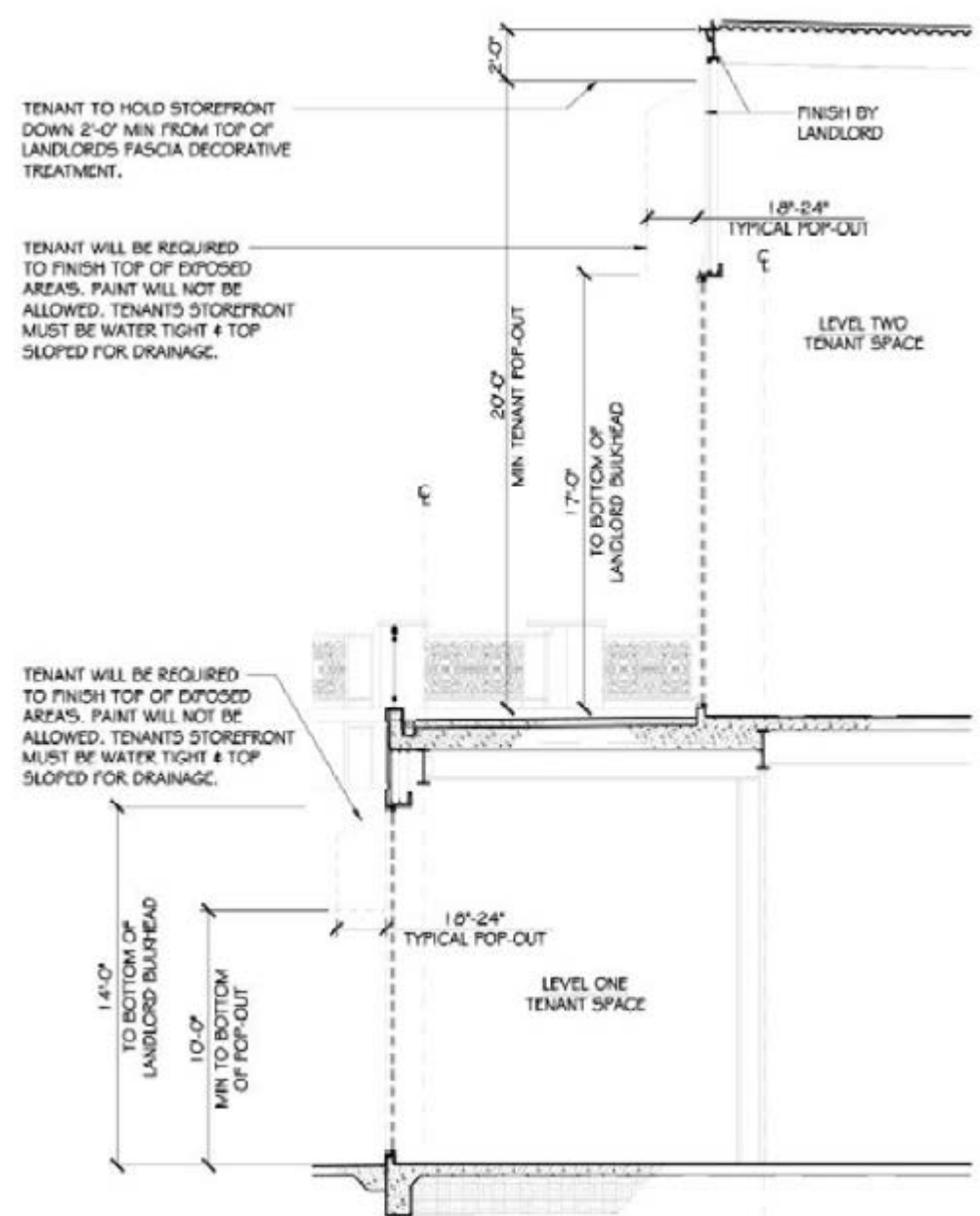
SECTION DETAIL
