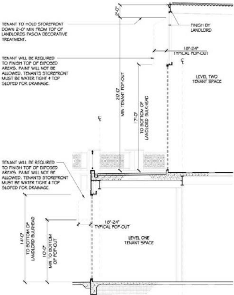
SECTION DETAIL CONTACT MALL T.C. FOR MORE INFORMATION - N.T.S.
