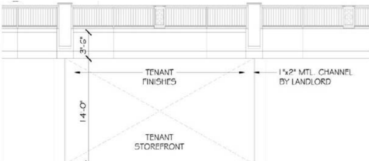
ELEVATION DETAIL CONTACT MALL T.C. FOR MORE INFORMATION - N.T.S.
