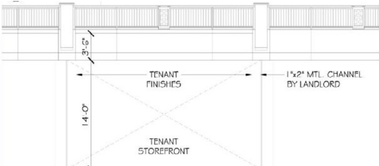
ELEVATION DETAIL CONTACT MALL T.C. FOR MORE INFORMATION - N.T.S.
