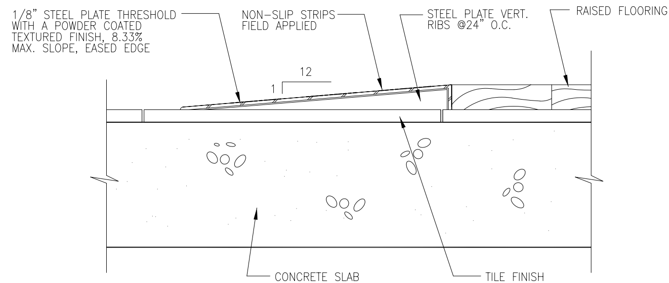
RAISED FLOOR THRESHOLD SCALE 6" = 1'-0"
