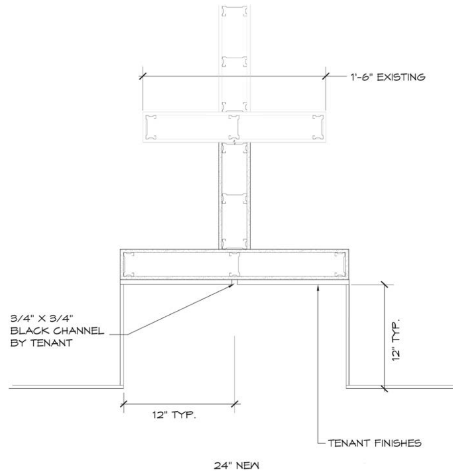
PLAN DETAIL @ NEUTRAL CHANNEL CONDITION SCALE: NTS
