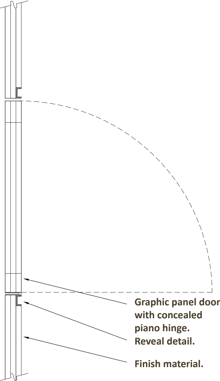
GRAPHIC FRAME DETAIL
