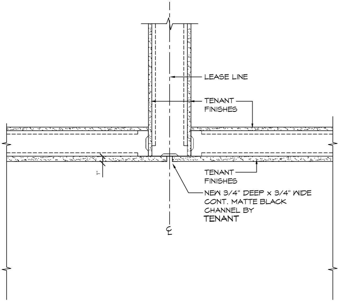
1 TYPICAL NEUTRAL CHANNEL DTL. TDC SCALE: 1-1/2"=1'-0"
