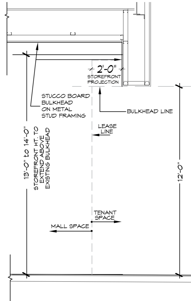
ZONE 2 WALL SECTION DETAIL
