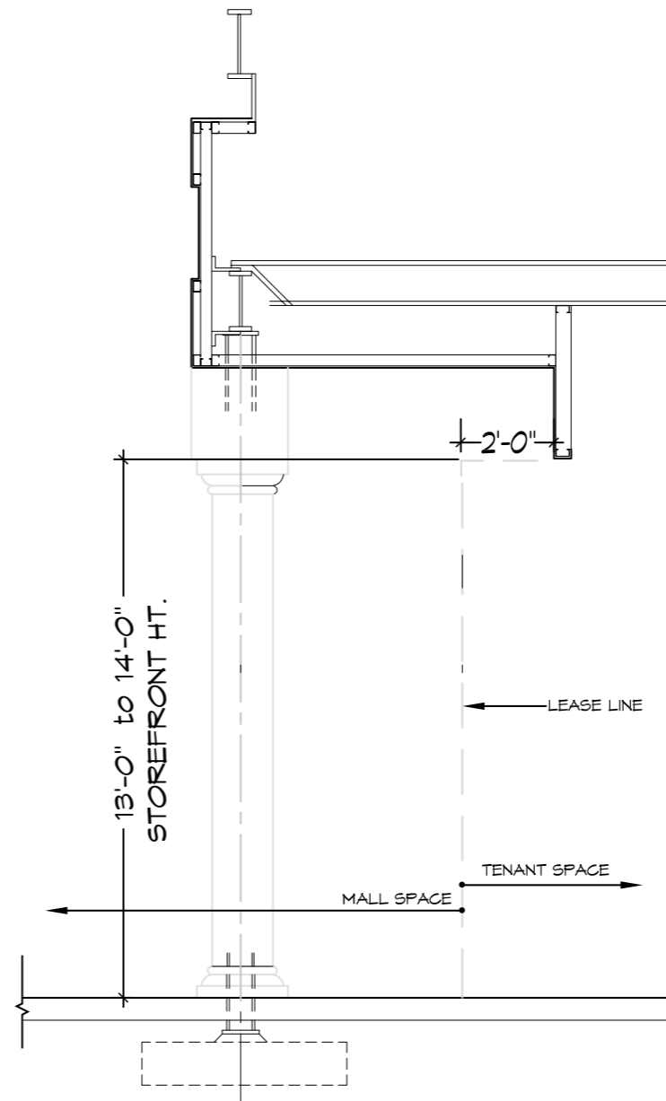
ZONE 3 WALL SECTION DETAIL
