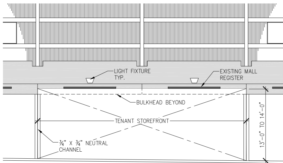
ZONE 1 ELEVATION DETAILS
