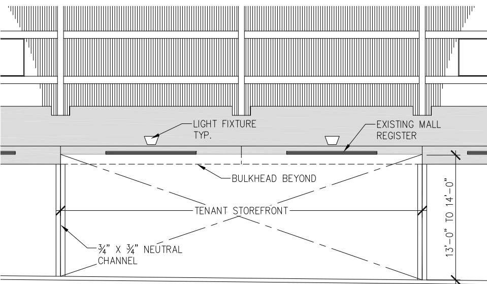
ZONE 1 ELEVATION DETAILS ZONE 1 ELEVATION DETAIL
