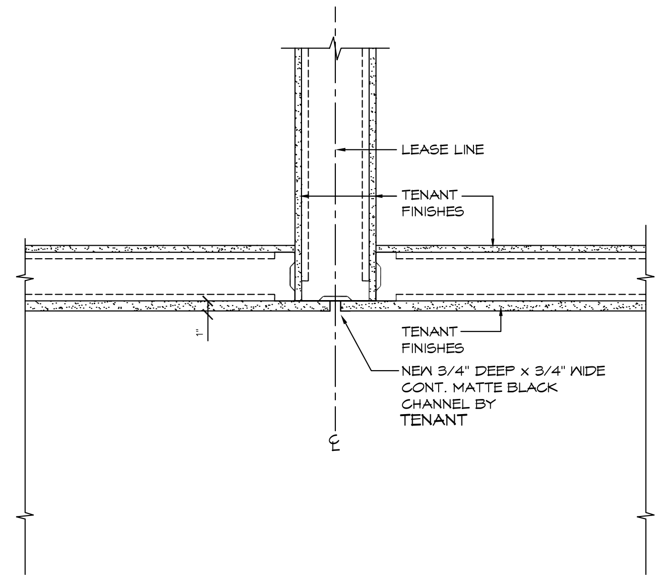
1 TYPICAL NEUTRAL CHANNEL DTL. TDC SCALE: 1-1/2"=1'-0"
