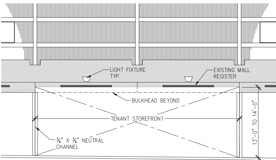
ZONE 1 ELEVATION DETAILS ZONE 1 ELEVATION DETAIL
