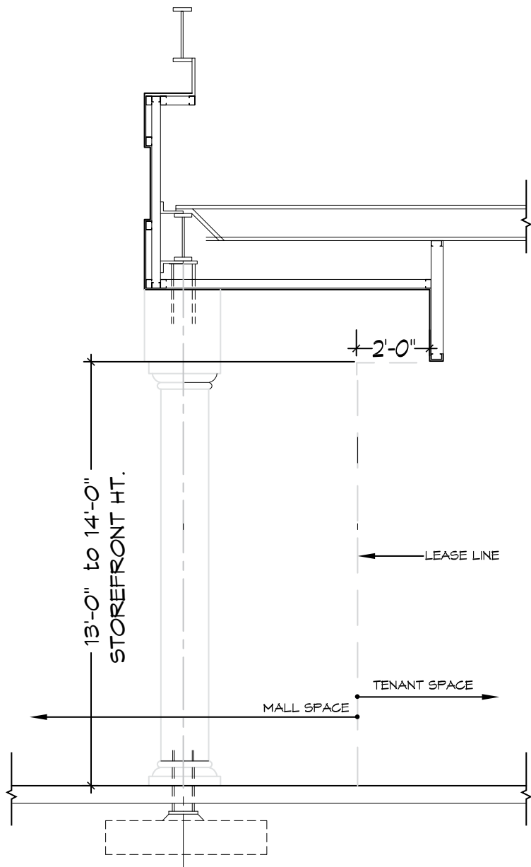
ZONE 3 WALL SECTION DETAIL
