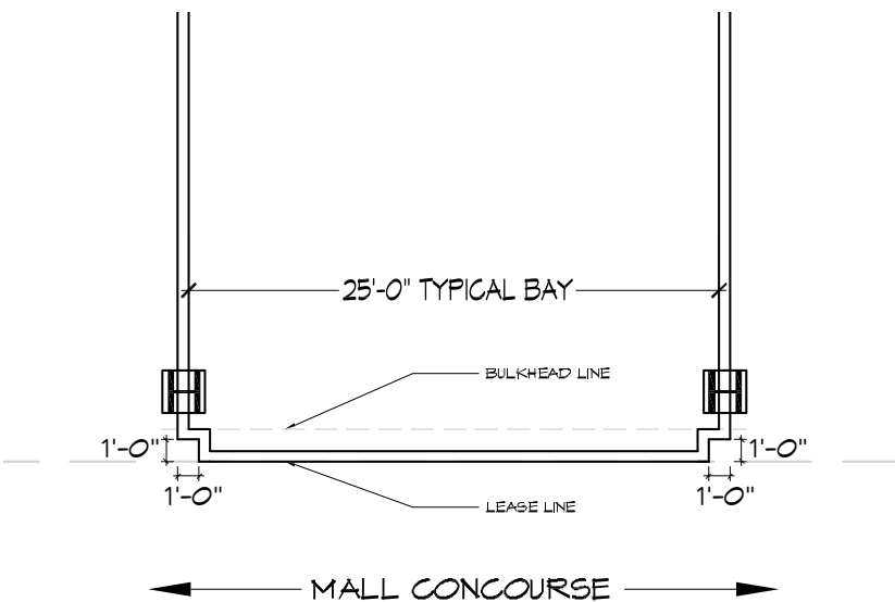
ZONE 1 PLAN DETAIL
