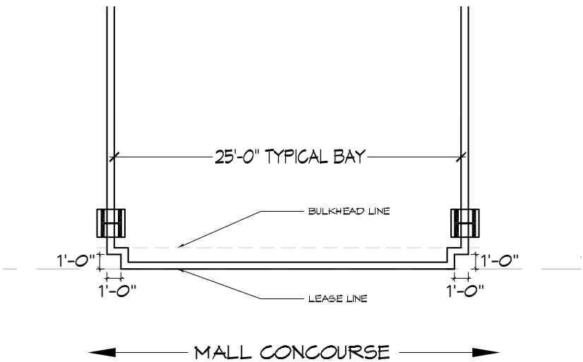
ZONE 3 PLAN DETAIL
