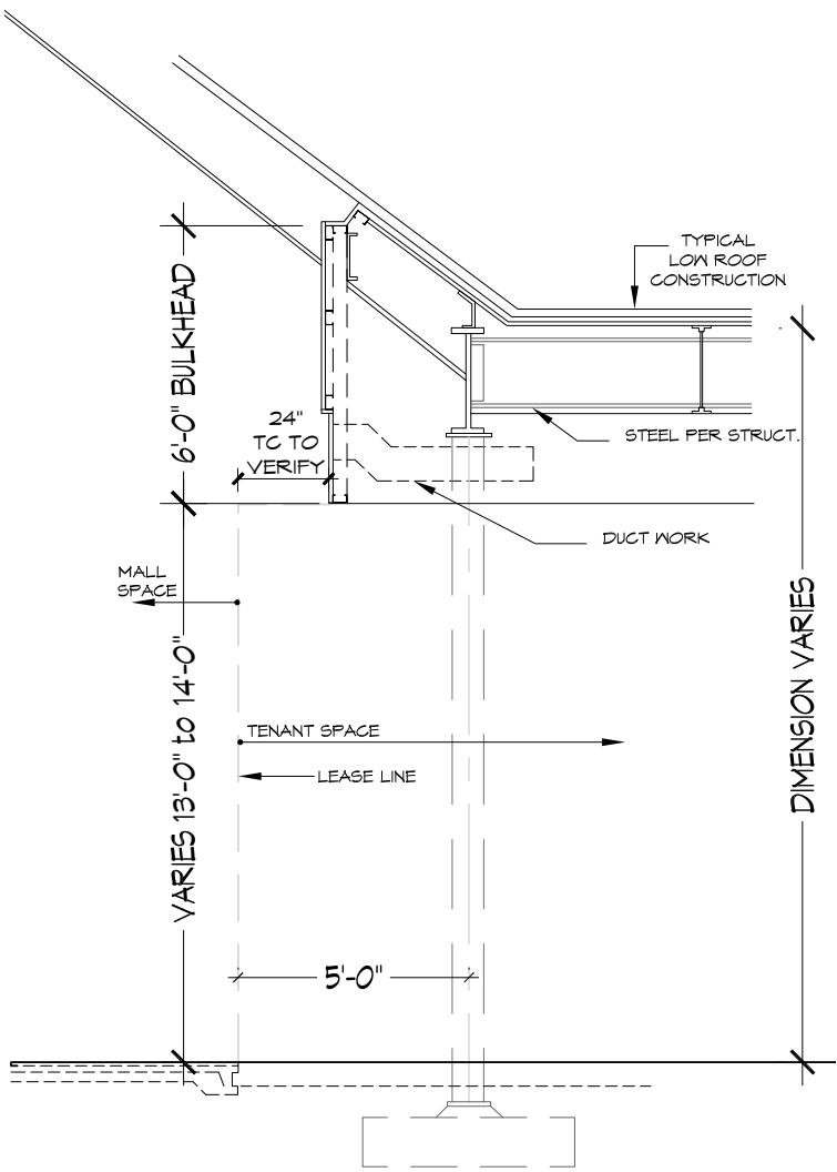
ZONE 1 WALL SECTION DETAIL
