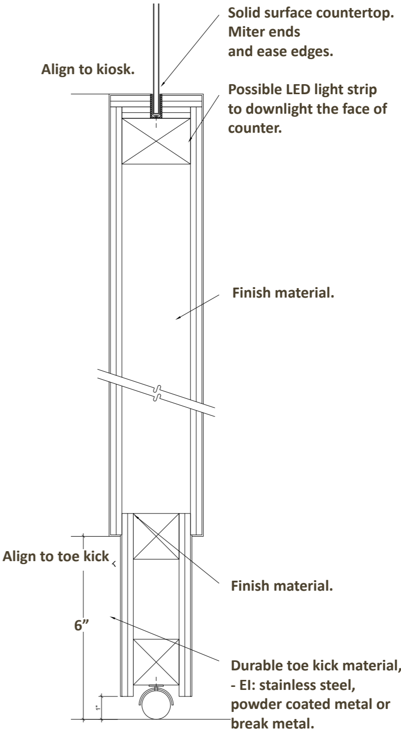
GATE DETAIL
