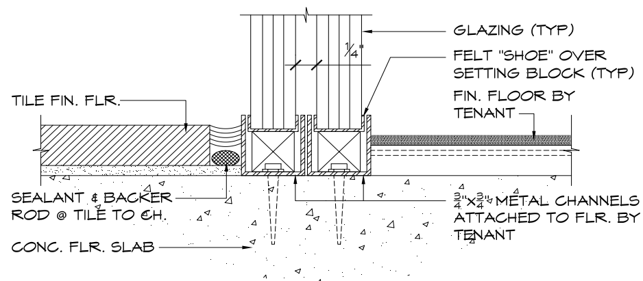
3 SECTION THRU STOREFRONT SILL @ SEISMIC JOINT a8 (HEAD DTL. SIMILAR)
