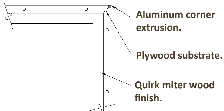
CORNER DETAIL
