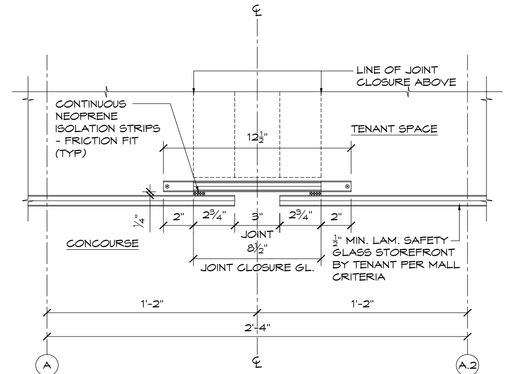
4 TENANT STOREFRONT SEISMIC JOINT PLAN DETAIL a8
