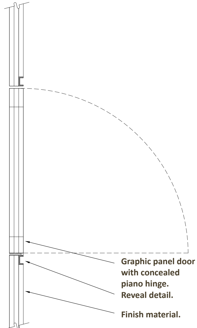
GRAPHIC FRAME DETAIL
