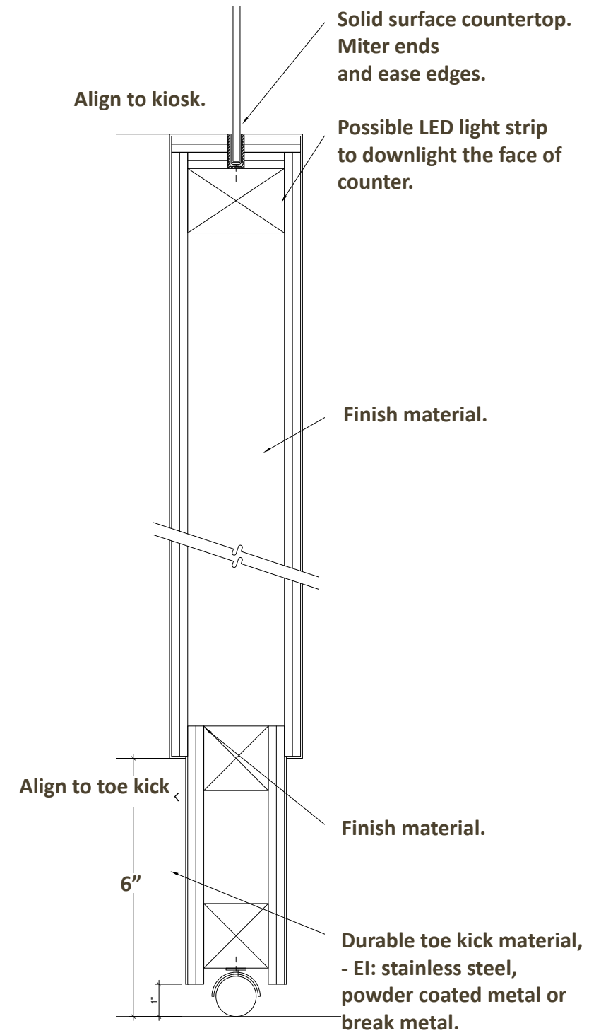
GATE DETAIL
