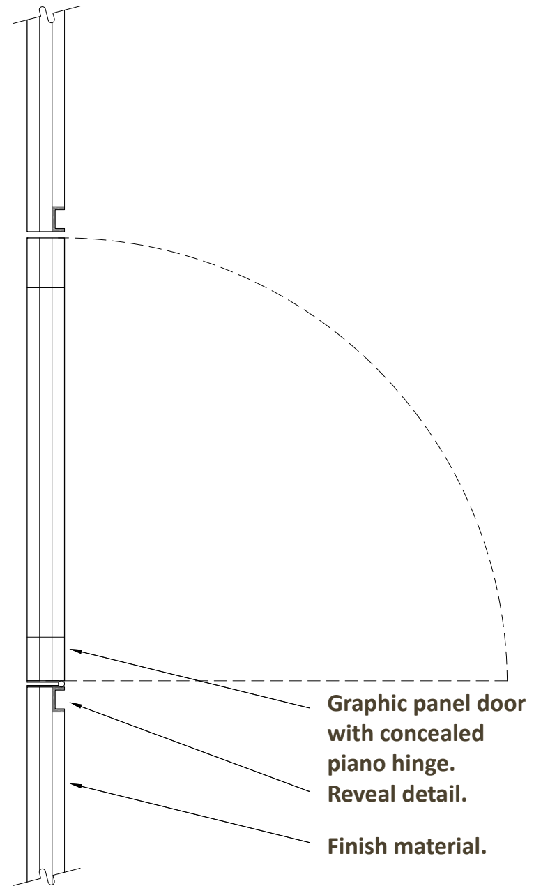
GRAPHIC FRAME DETAIL
