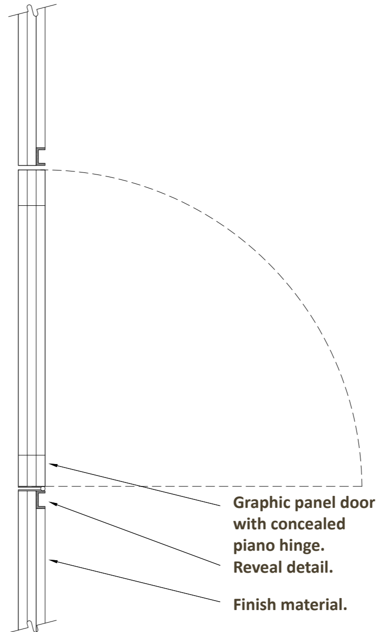
GRAPHIC FRAME DETAIL
