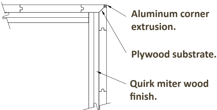
CORNER DETAIL
