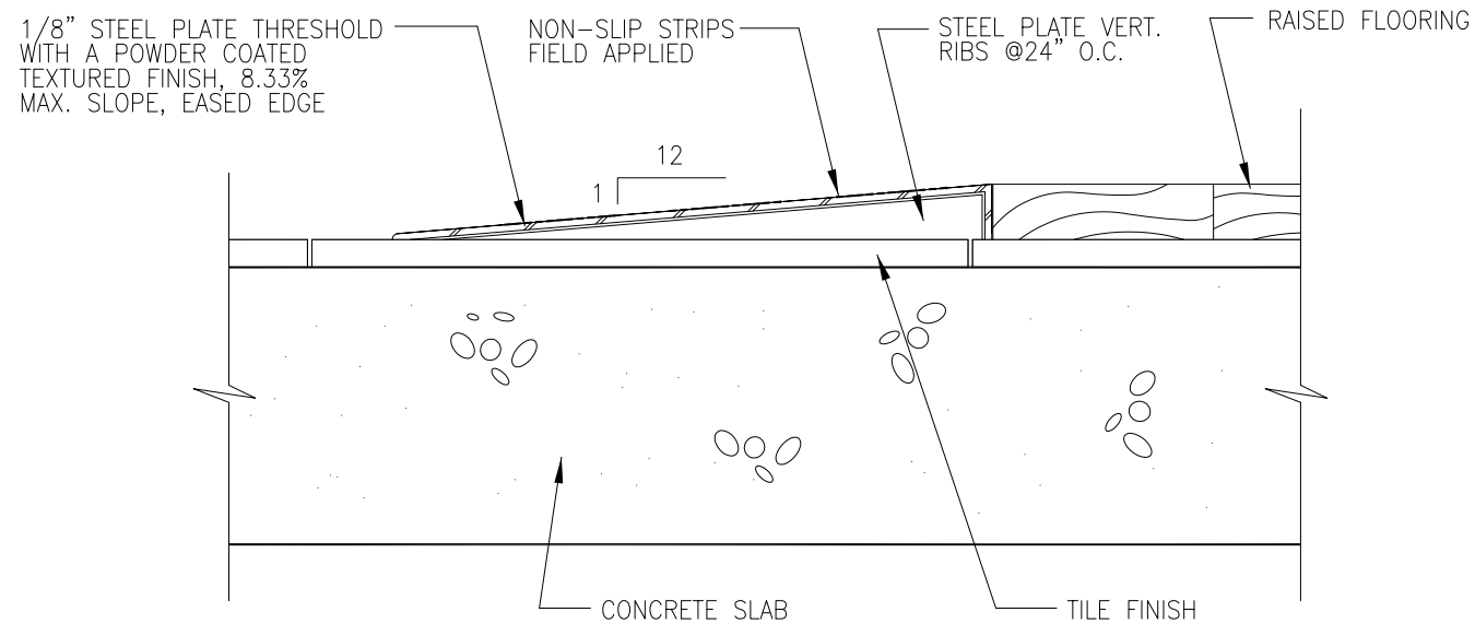
RAISED FLOOR THRESHOLD
