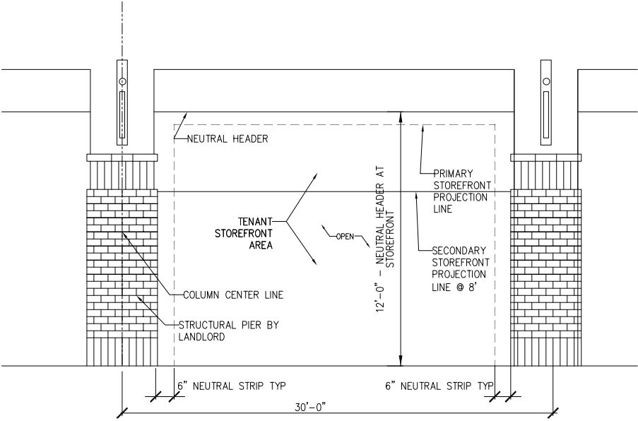
TENANT STOREFRONT ZONES - ZONE 1 - LEVEL ONE STOREFRONT ELEVATION
