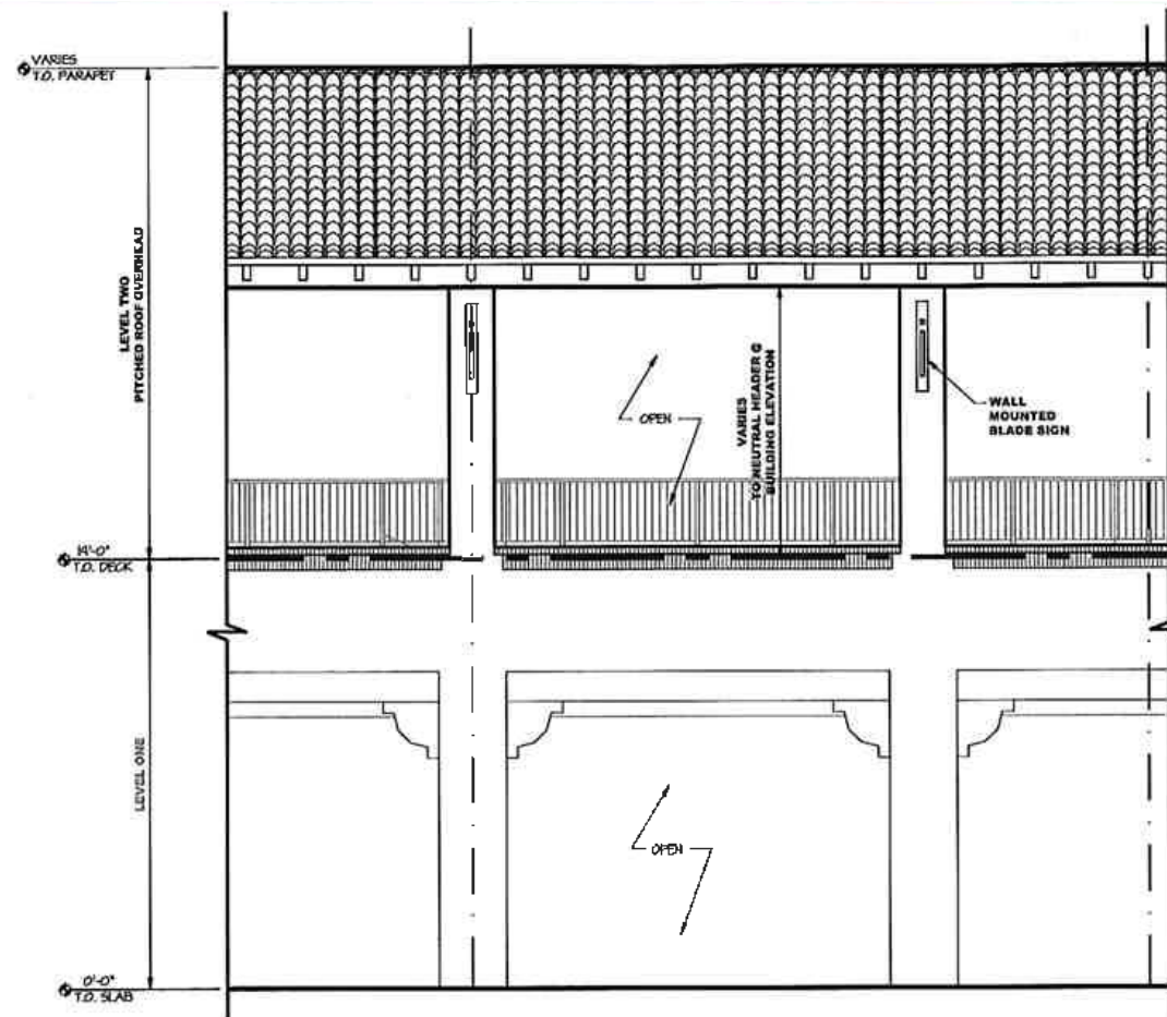
TENANT STOREFRONT ZONES - ZONE 5 - LEVEL TWO BUILDING ELEVATION
