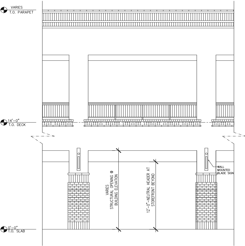
TENANT STOREFRONT ZONES - ZONE 1 - LEVEL ONE BUILDING ELEVATION
