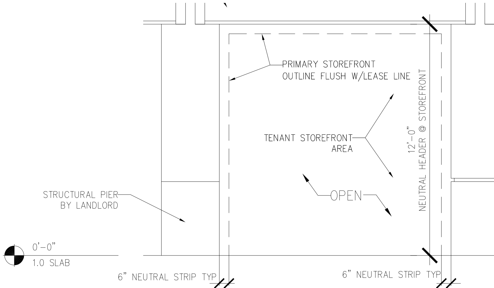
TENANT STOREFRONT ZONES - ZONE 2 - LEVEL ONE BUILDING ELEVATION
