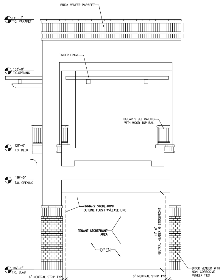
TENANT STOREFRONT ZONES - ZONE 6 - LEVEL TWO BUILDING ELEVATION
