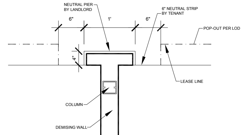
TYPICAL NEUTRAL PIER DETAIL
