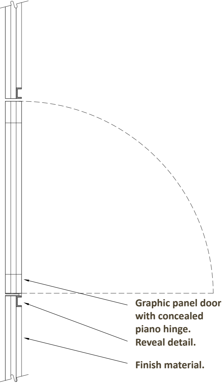
GRAPHIC FRAME DETAIL
