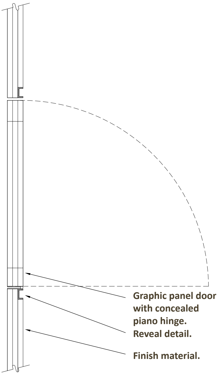
GRAPHIC FRAME DETAIL
