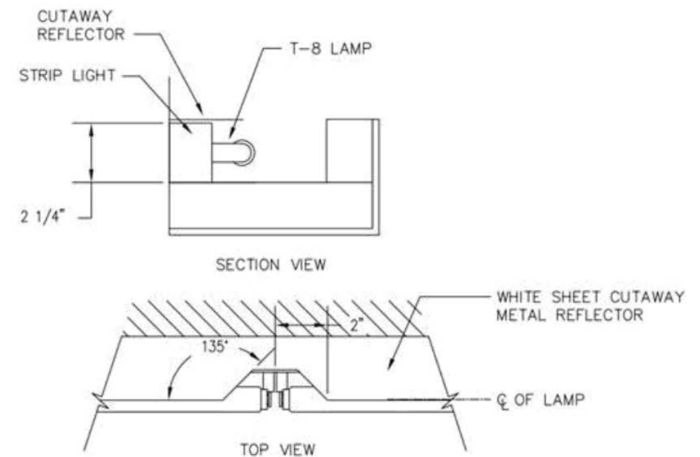
MOUNTING FOR TYPE F7
