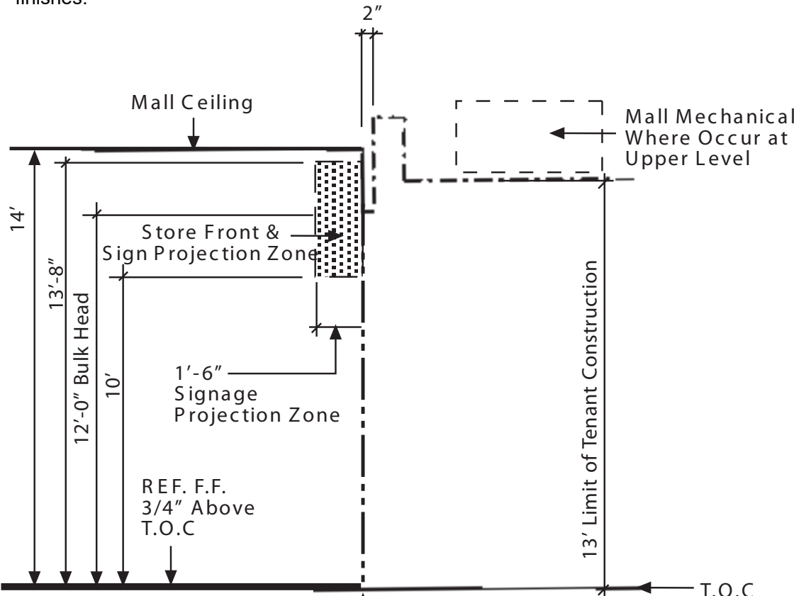
SECTION
