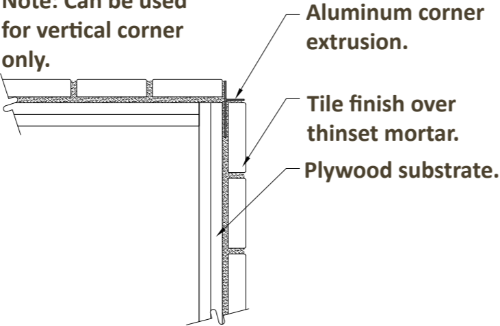
CORNER DETAIL
